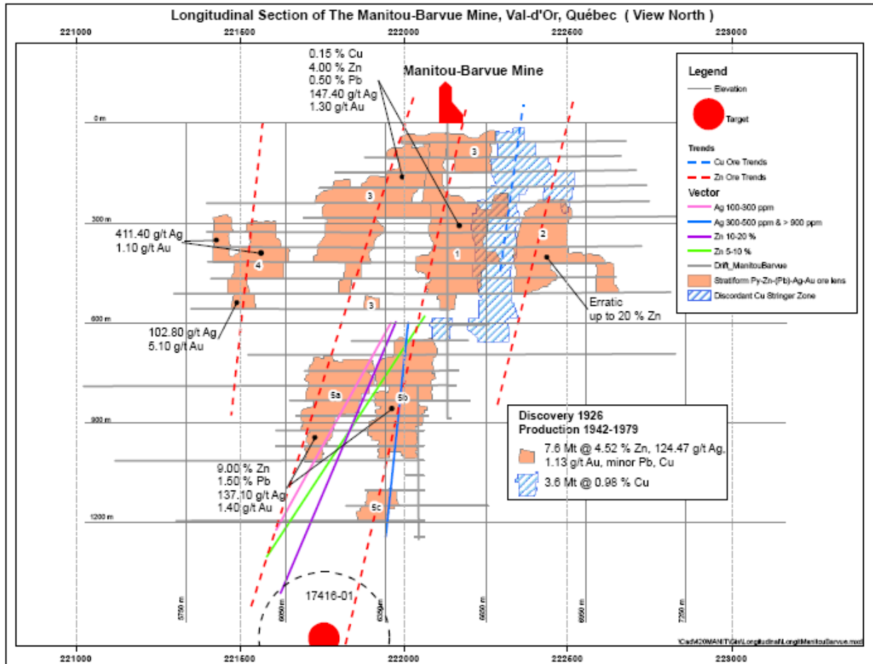
Figure 1: Longitudinal Section of the Past-Producing Manitou-Barvue Mine, Val d'Or Québec.
